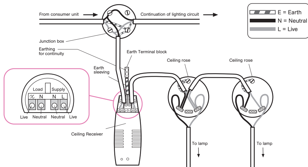
Mains Voltage installation example - Fig 3
