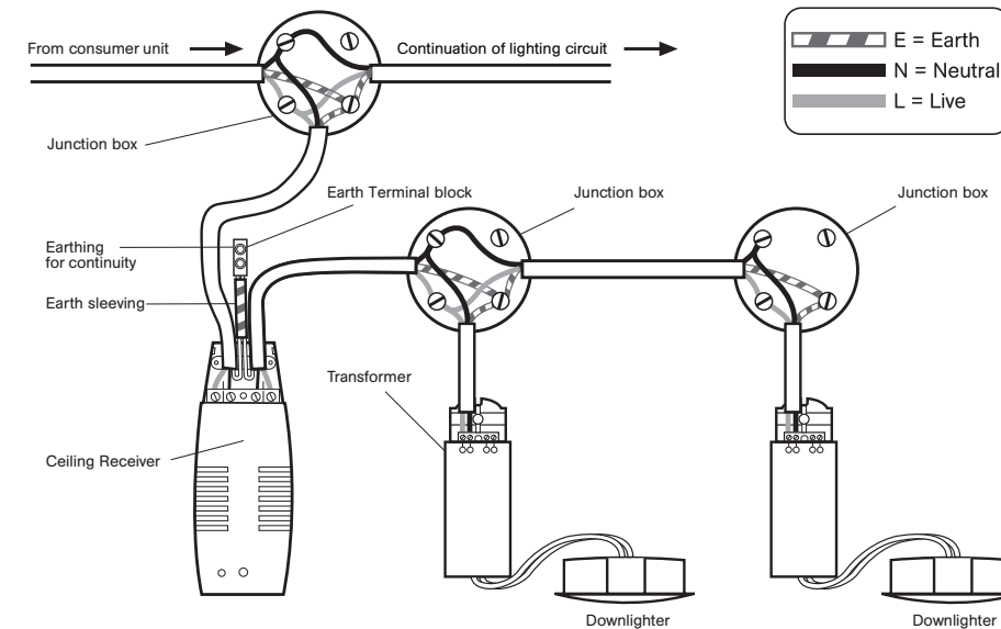
Low Voltage installation example – Fig 2
